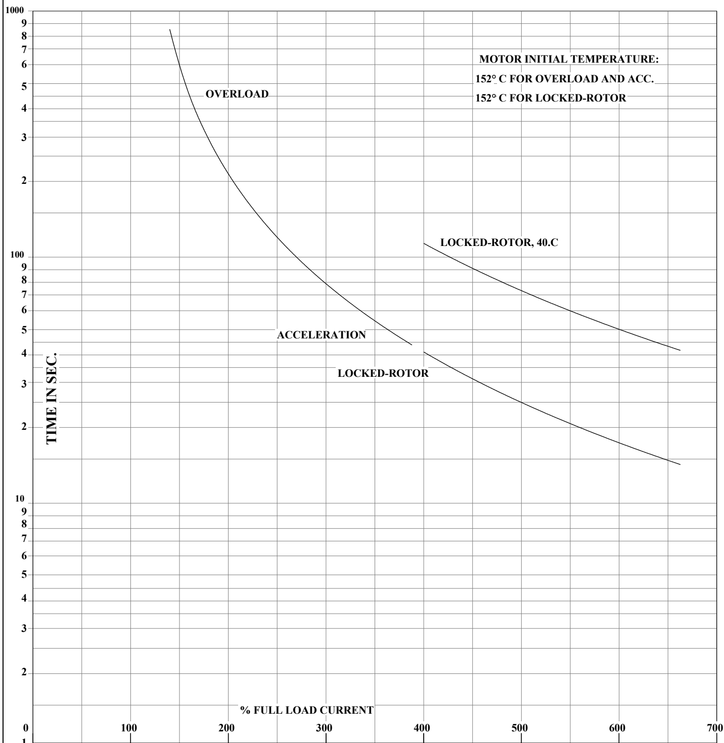
THERMAL LIMIT CURVE XE MOTOR-TYPICAL DATA-NEMA NOM. EFF. 96.2 PCT.
