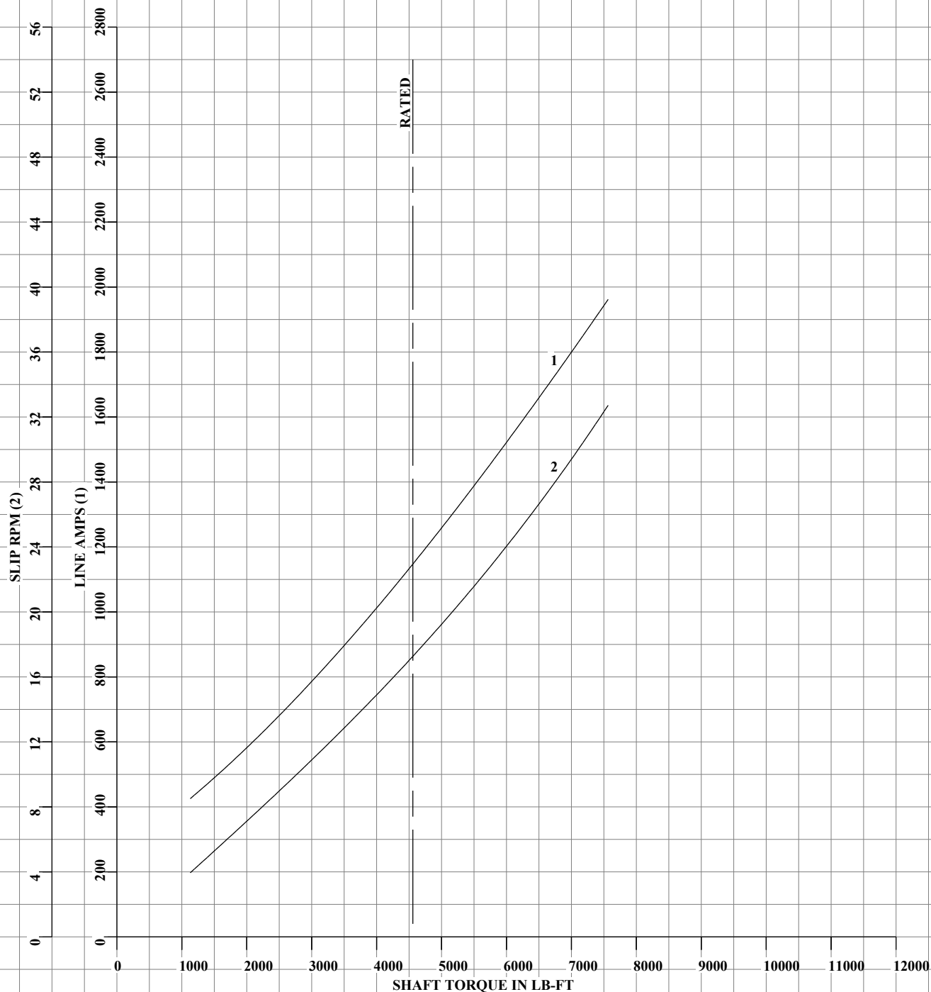
TYPICAL DATA LOAD PERFORMANCE (CONSTANT V/HZ RANGE)
