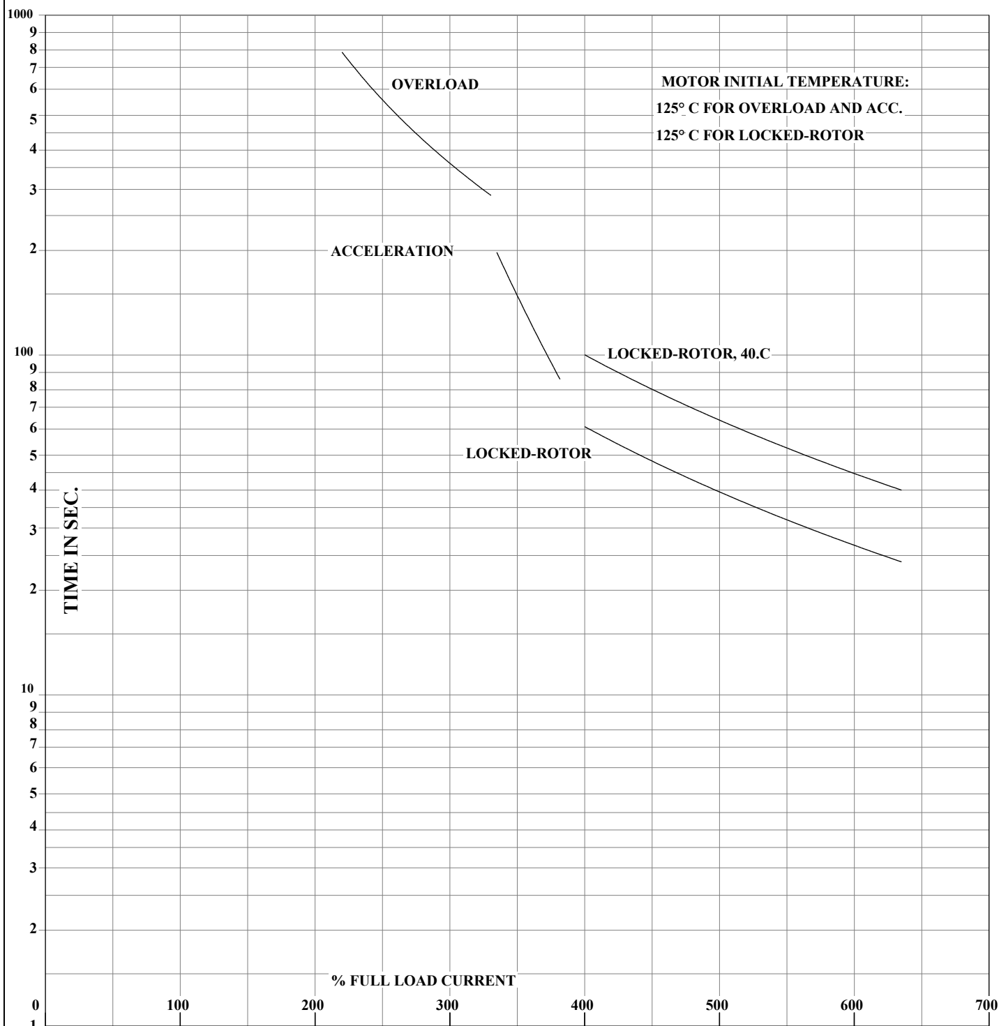
THERMAL LIMIT CURVE TYPICAL DATA-NEMA NOM. EFF. 95.4 PCT.
