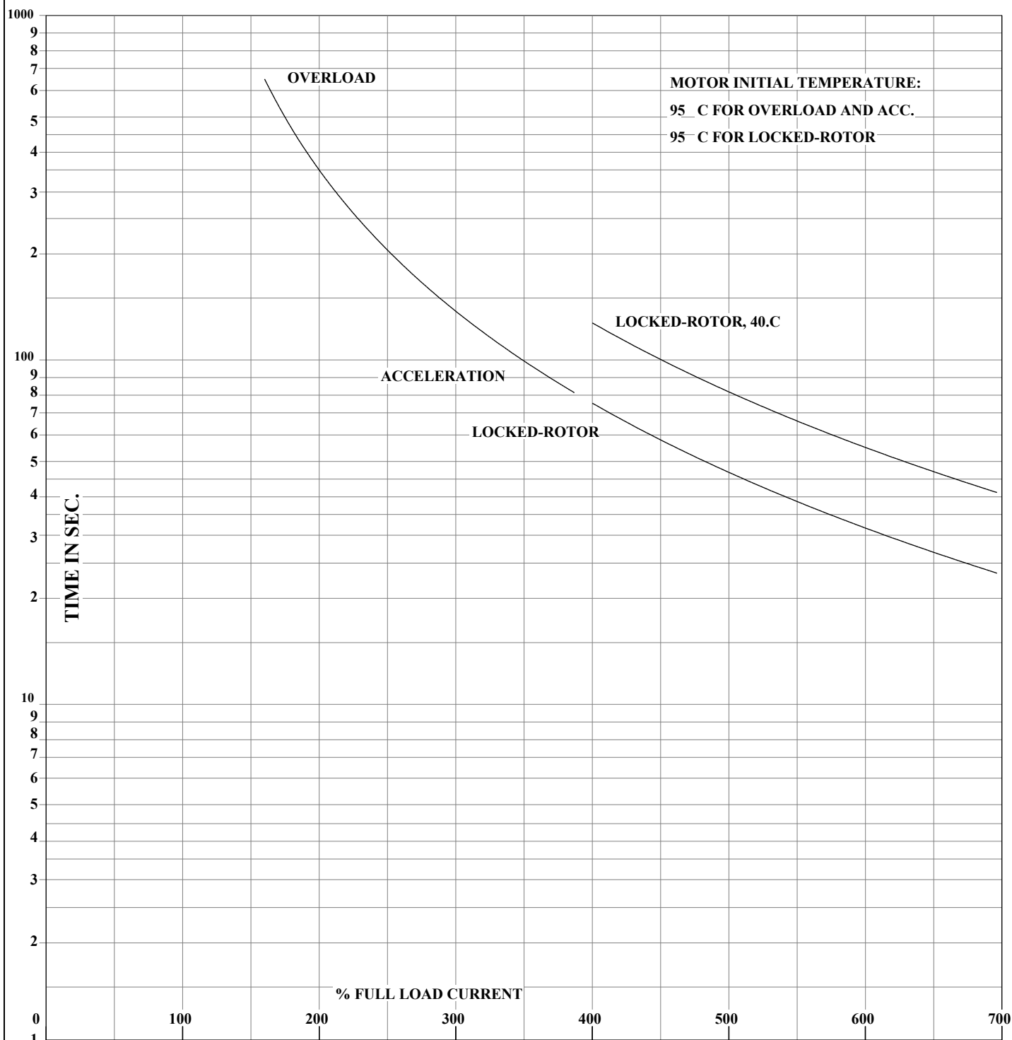
THERMAL LIMIT CURVE XE MOTOR-TYPICAL DATA-NEMA NOM. EFF. 94.5 PCT.
