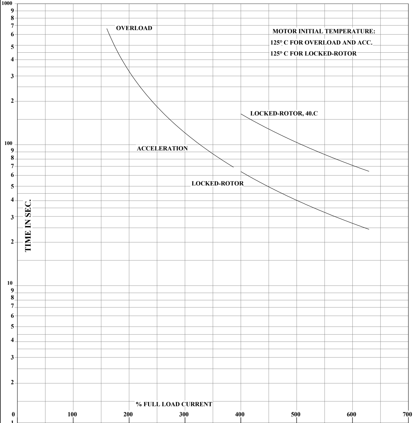
THERMAL LIMIT CURVE XE MOTOR - NEMA NOM. EFF. 95.0%
