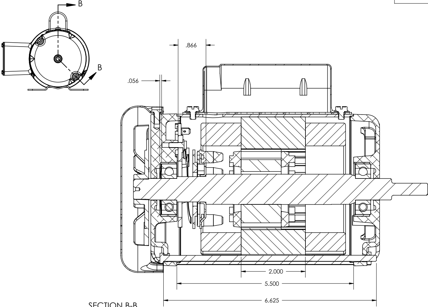
SECTION B-B
